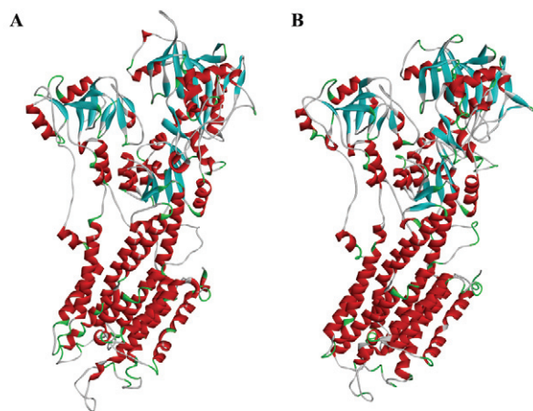
Fig. 1: three-dimensional structure of the mammalian Ca 2+ -ATPase 1IWO (A) and parasite PfATP6 model (B).
