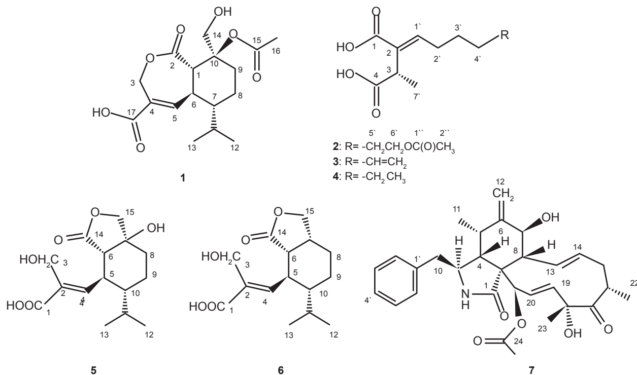
Fig. 2: structures of compounds 1-7 isolated from the endophytic fungus Nectria pseudotrachia .
