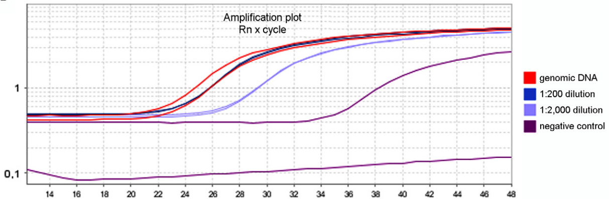
Amplification plots from sample dilution test for real-time polymerase chain reaction. A: graphical representation of real-time amplification from all tested dilution points; B: graphical representation of real-time amplification showing the two most reliable dilutions.
