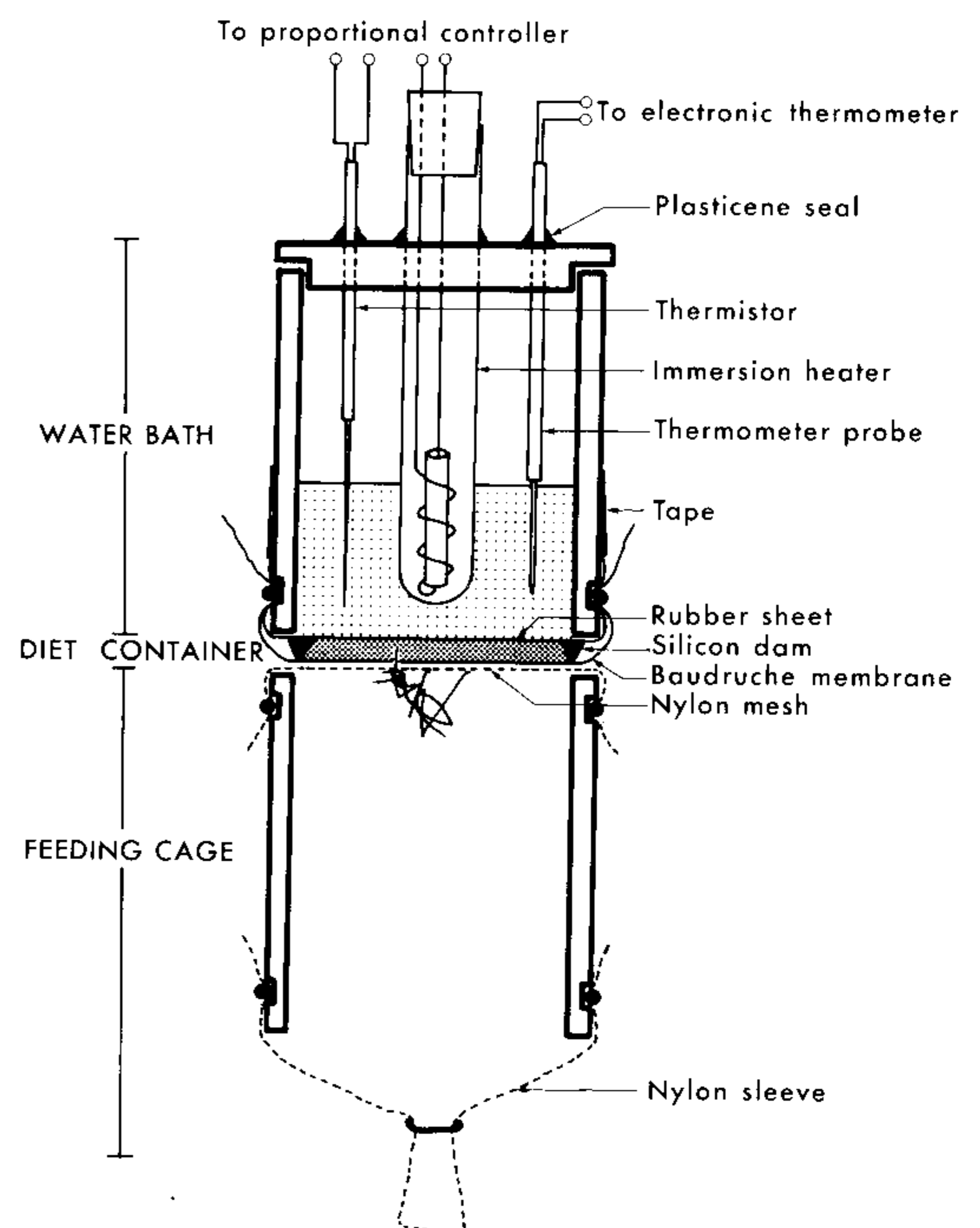
Fig. 1: Feeding apparatus for feeding small volumes of radioactive or expensive diets to mosquitoes and other blood-sucking insects (Friend & Hewson, 1978).
